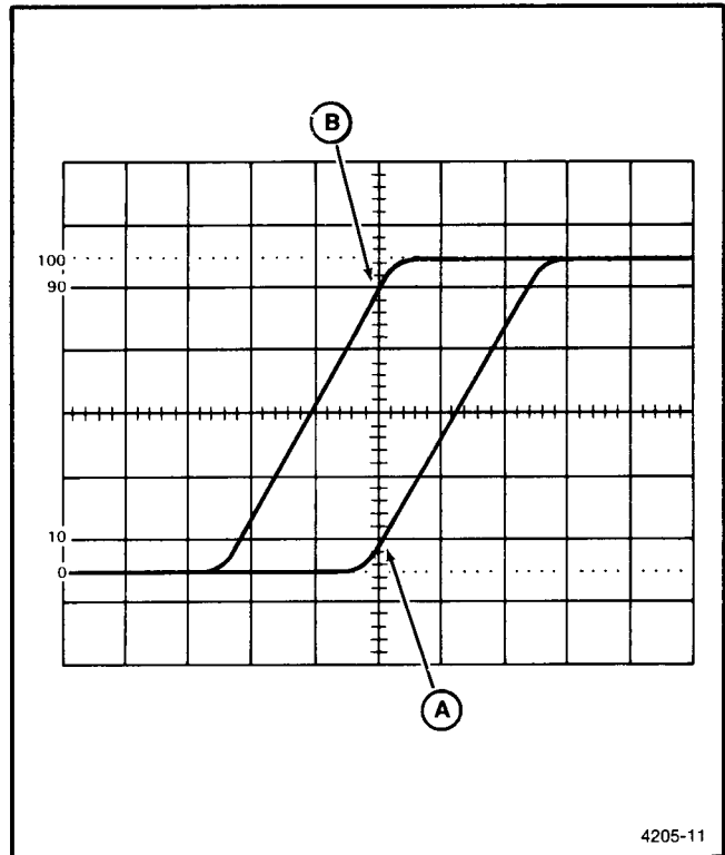
Fig. 4-7. Rise time.
