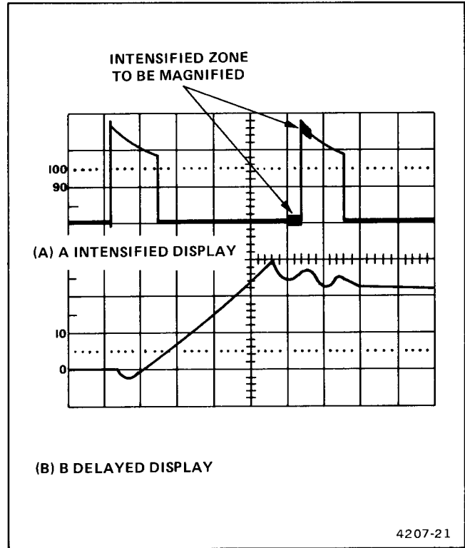
Fig. 4-5. Delayed-sweep magnification.
