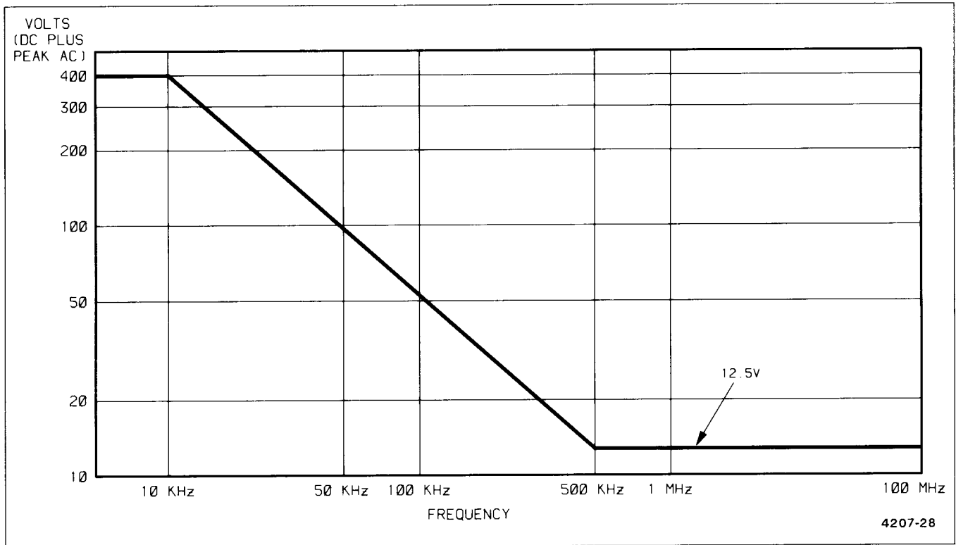
Fig. 1-1. Maximum input voltage vs frequency derating curve for CH 1 OR X & DMM, CH 2 OR Y, and EXT INPUT connectors.
