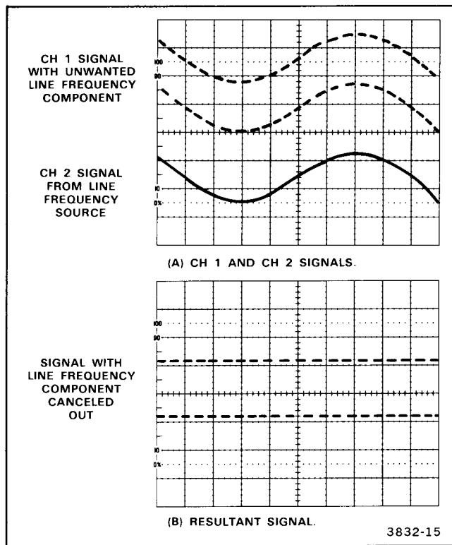
Fig. 4-3. Common-mode rejection.
