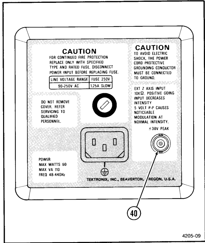
Fig. 2-9. Rear-panel connector.
