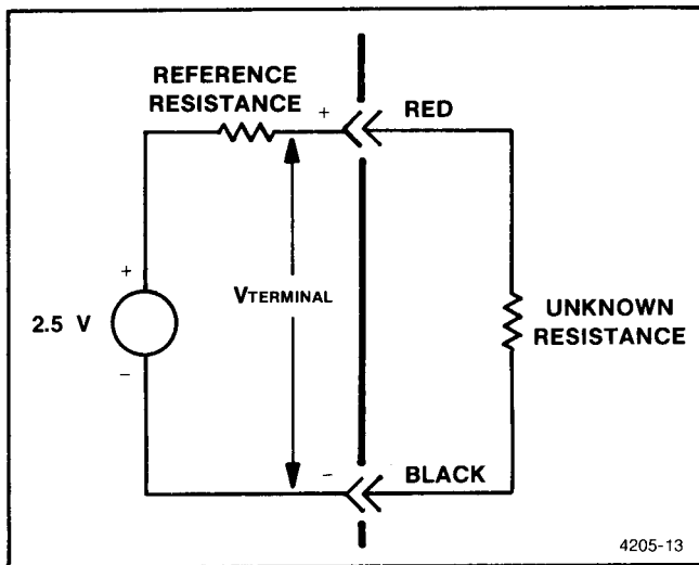
Fig. 4-9. Resistance measurement technique.
