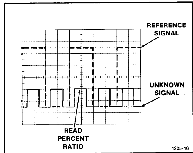
Fig. 4-4. Voltage ratios.
