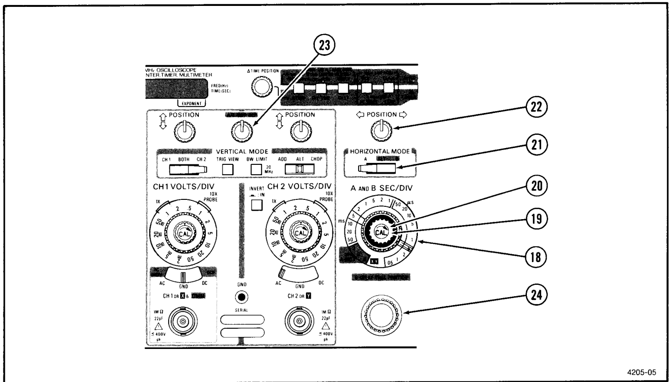
Fig. 2-5. Horizontal controls.
