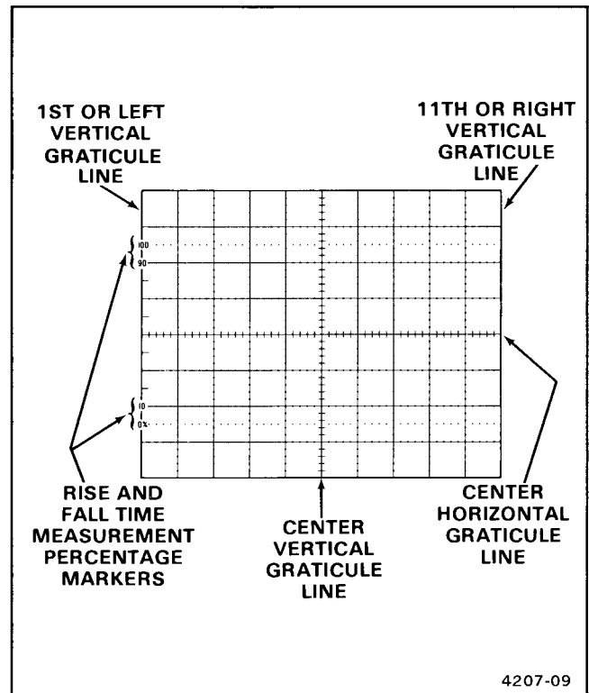
Fig. 3-1. Graticule measurement markings.
