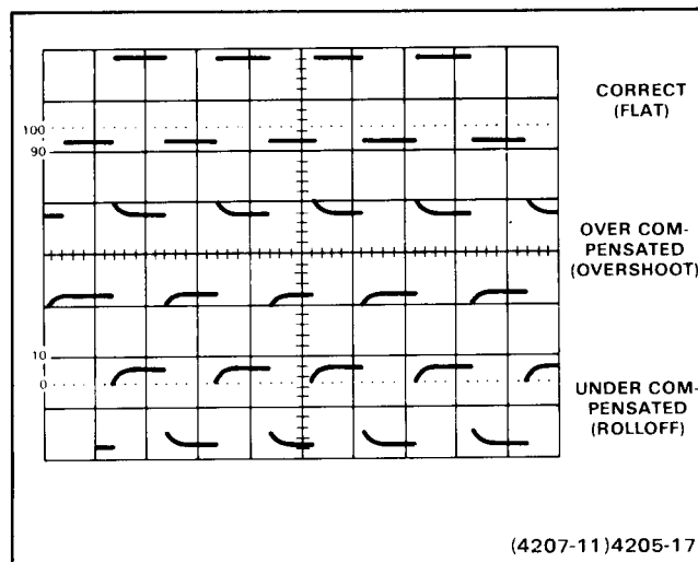
Fig. 3-2. Probe compensation.
